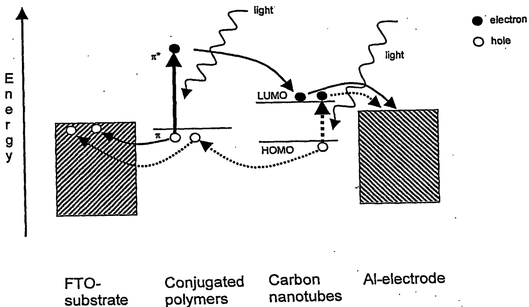
Fig. 2: Schematic band diagram and different excitation processes of and in a carbon nanotube based photovoltaic device according to the present invention.
